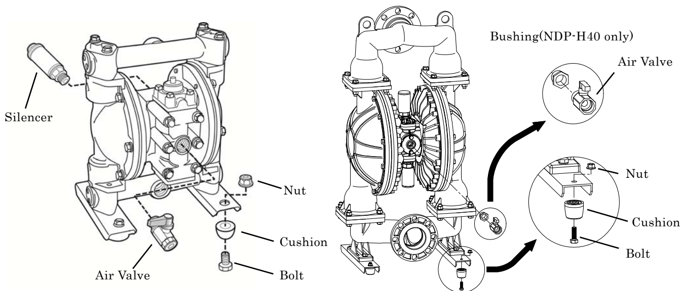
NDP-H40~NDP-H80 Type
